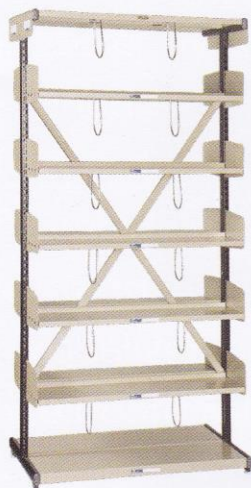
S - 317 N 925W x 546D x 1969H mm.
