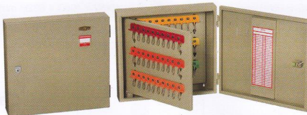
KB - 860 405W x 80D x 375H mm.
